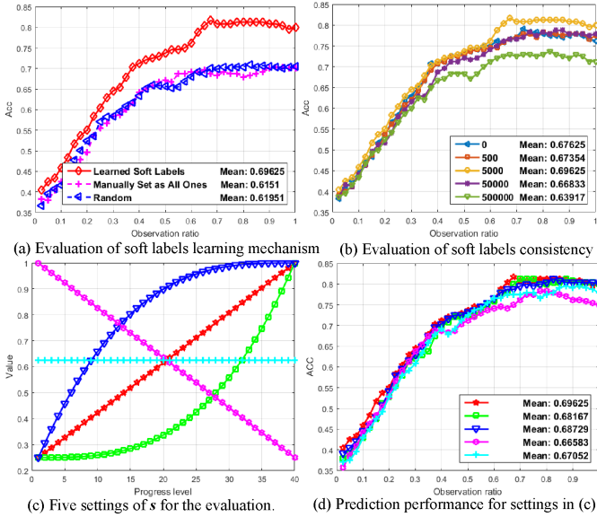
Fig. 6. More evaluations on the system performance.
