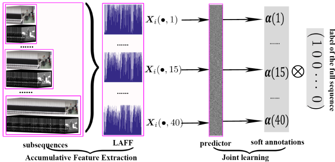
Fig. 2. A graphic illustration of our soft regression model. \otimes is Kronecker product.
