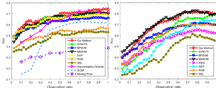
Fig. 4. Comparison results on ORGBD (left) and SYSU 3DHOI (right) sets.
