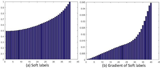
Fig. 5. Example soft labels learned on SYSU 3DHOI set. The vertical axis indicates the values for the soft labels and the horizontal axis is the index of subsequence.
